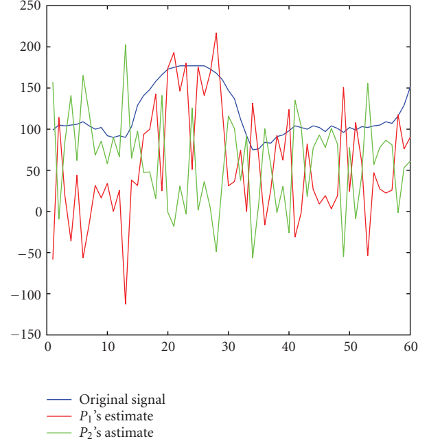
FIGURE 2: Original signal and least-square estimates in secure inner product.
