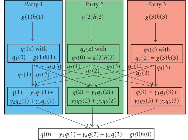
FIGURE 1: This diagram shows how three parties can share the secret g(0)h(0) based on the locally computed products g(1)h(1), g(2)h(2) , and g(3)h(3) .
